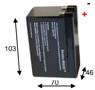
Battery terminal position
