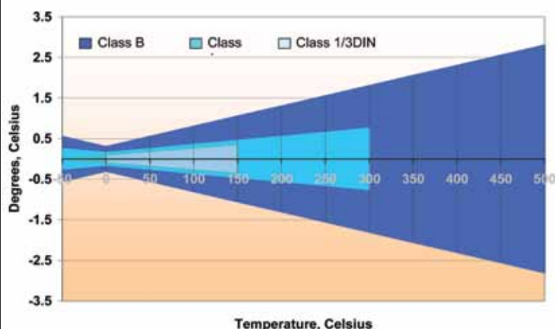
Thin Film RTD Accuracy Classes
